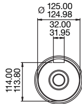
SHAFT END DETAIL
