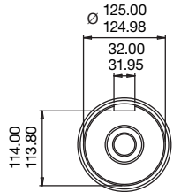
SHAFT END DETAIL
